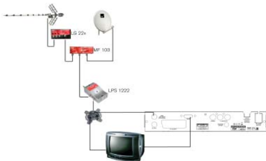
Example 3 - Combined with terrestrial
