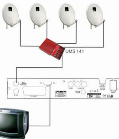
Example 2 - DISEqC switches
